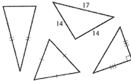
Isosceles triangles
