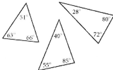
Acute triangles
