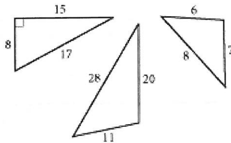
Scalene triangles
