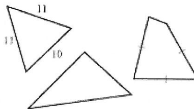
Not equilateral triangles
