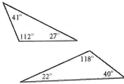
Obtuse triangles
